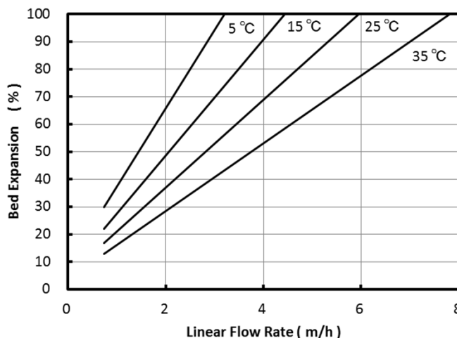
Fig. 2 Bed Expansion of SA11A
