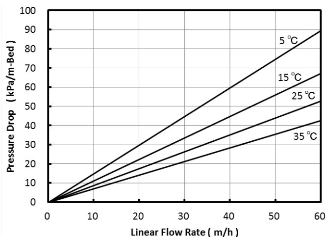
Fig. 1 Pressure Drop of PA312L
