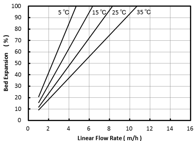
Fig. 2 Bed Expansion of PA312L
